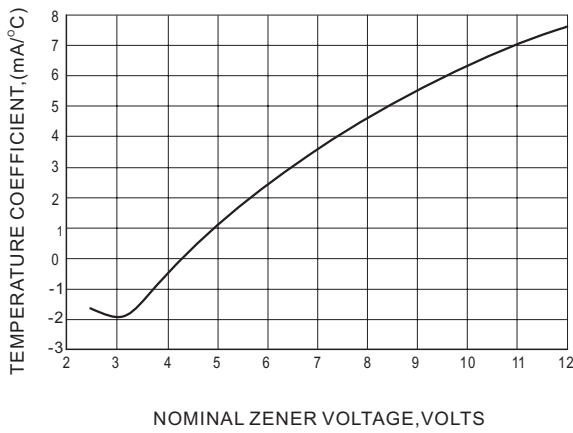
Fig. 1 TEMPERATURE COEFFICIENTS
