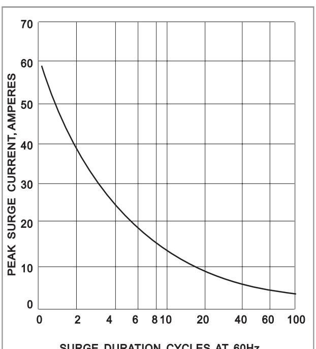
FIG.4-NON-RECURRENT SURGE RATING
