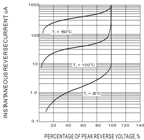
Fig.3-TYPICAL REVERSE CHARACTERISTIC
