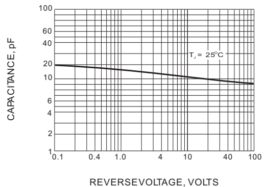
Fig.5-TYPICAL JUNCTION CAPACITANCE
