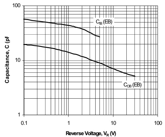
Fig. 4. Typical Capacitances
