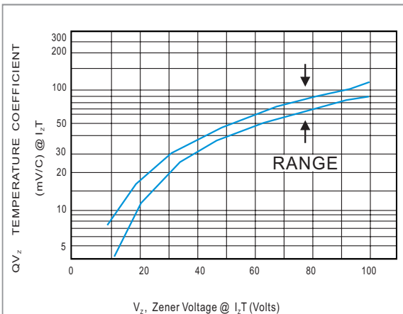
Fig.2 Temperature Coefficient-Range For units 10 to 100 volts
