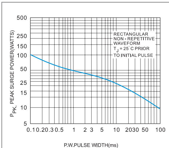
FIGURE 2. MAXIMUM SURGE POWER
