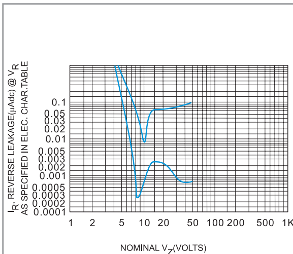
FIGURE 3. TYPICAL REVERSE LEAKAGE
