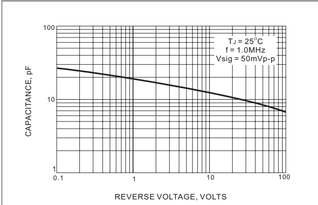
FIG. 1 TYPICAL JUNCTION CAPACITANCE
