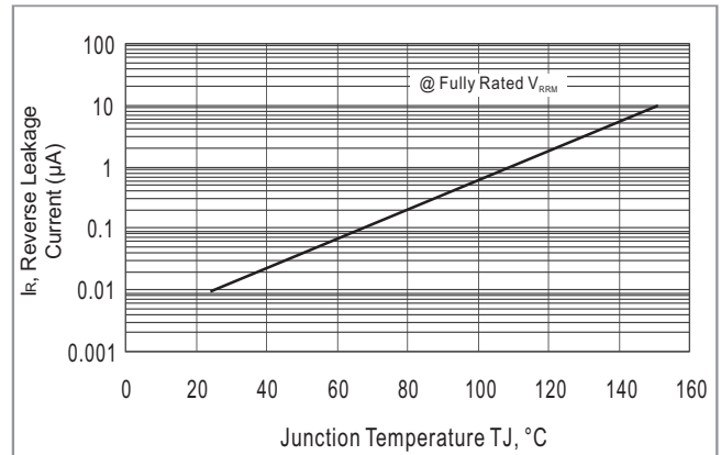
FIG-2 TYPICAL LEAKAGE CURRENT vs JUNCTION TEMPERATURE
