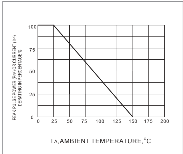
Fig.2 DERATING CURVE
