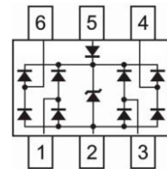
Fig.200(Top View)
