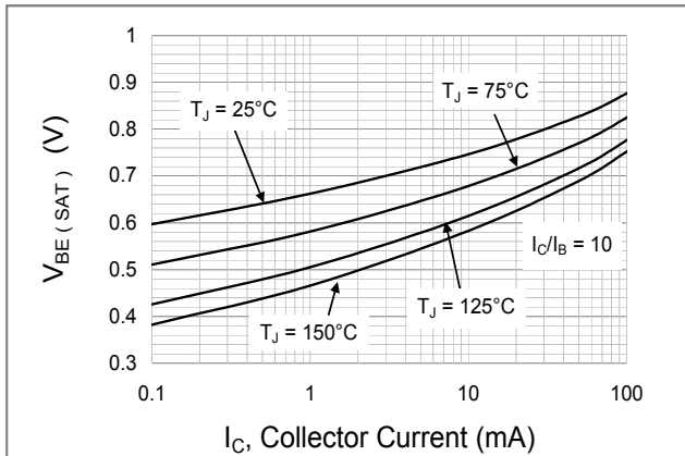
Fig.1 Base-Emitter Saturation Voltage
