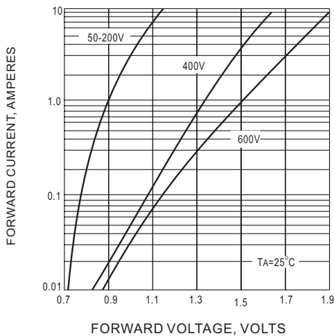
Fig.3 FORWARD CHARACTERISTICS
