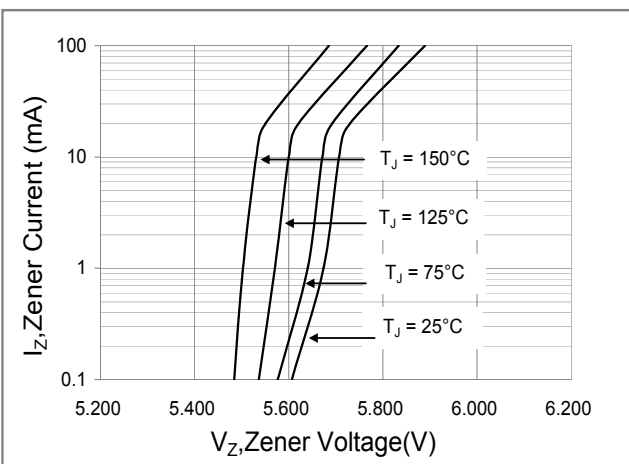
Fig.5 Typical Zener Characteristics
